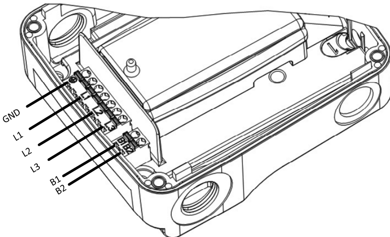
Figure 3: Electrical scheme
